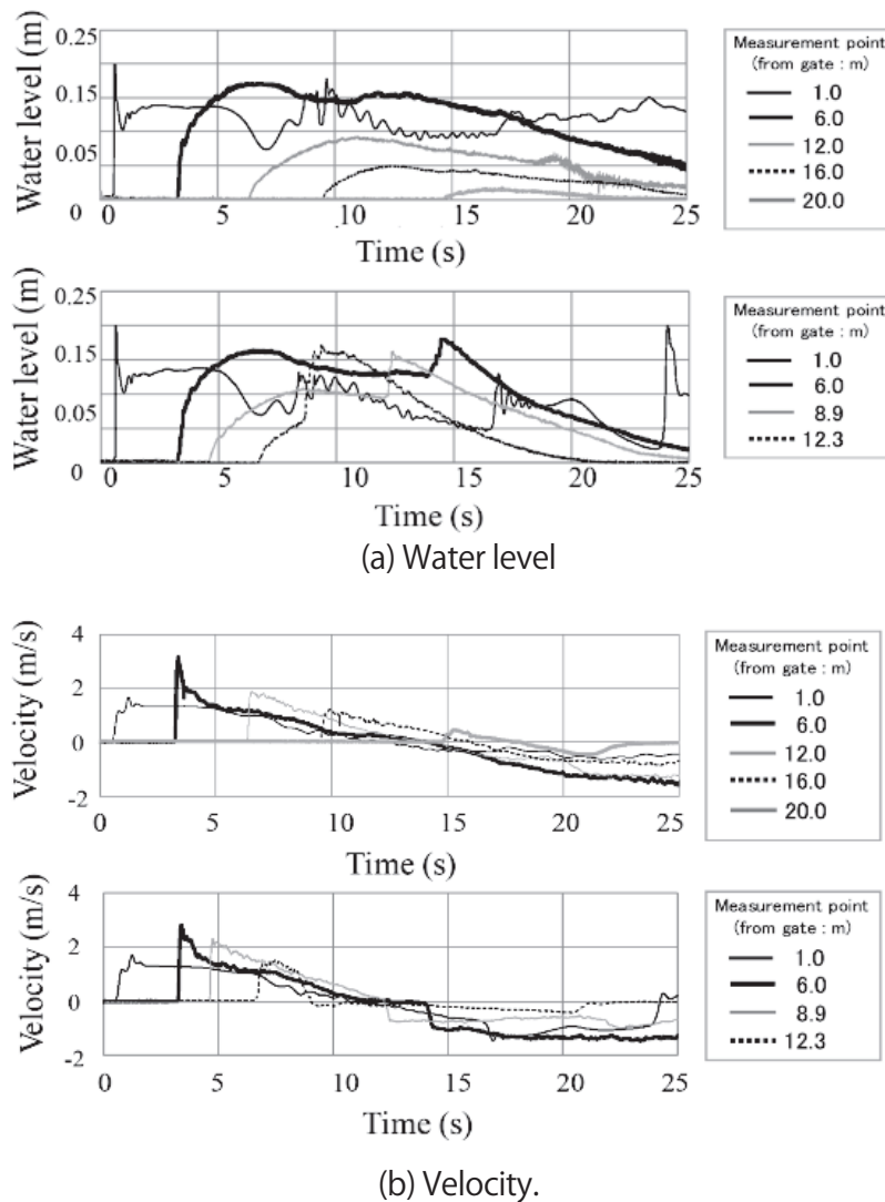
Figure 3. Water level and velocity at each measurement point in the fixed bed cases: (upper panels) nonreturn flow and (lower panels) return flow (i.e., reflection wall)
