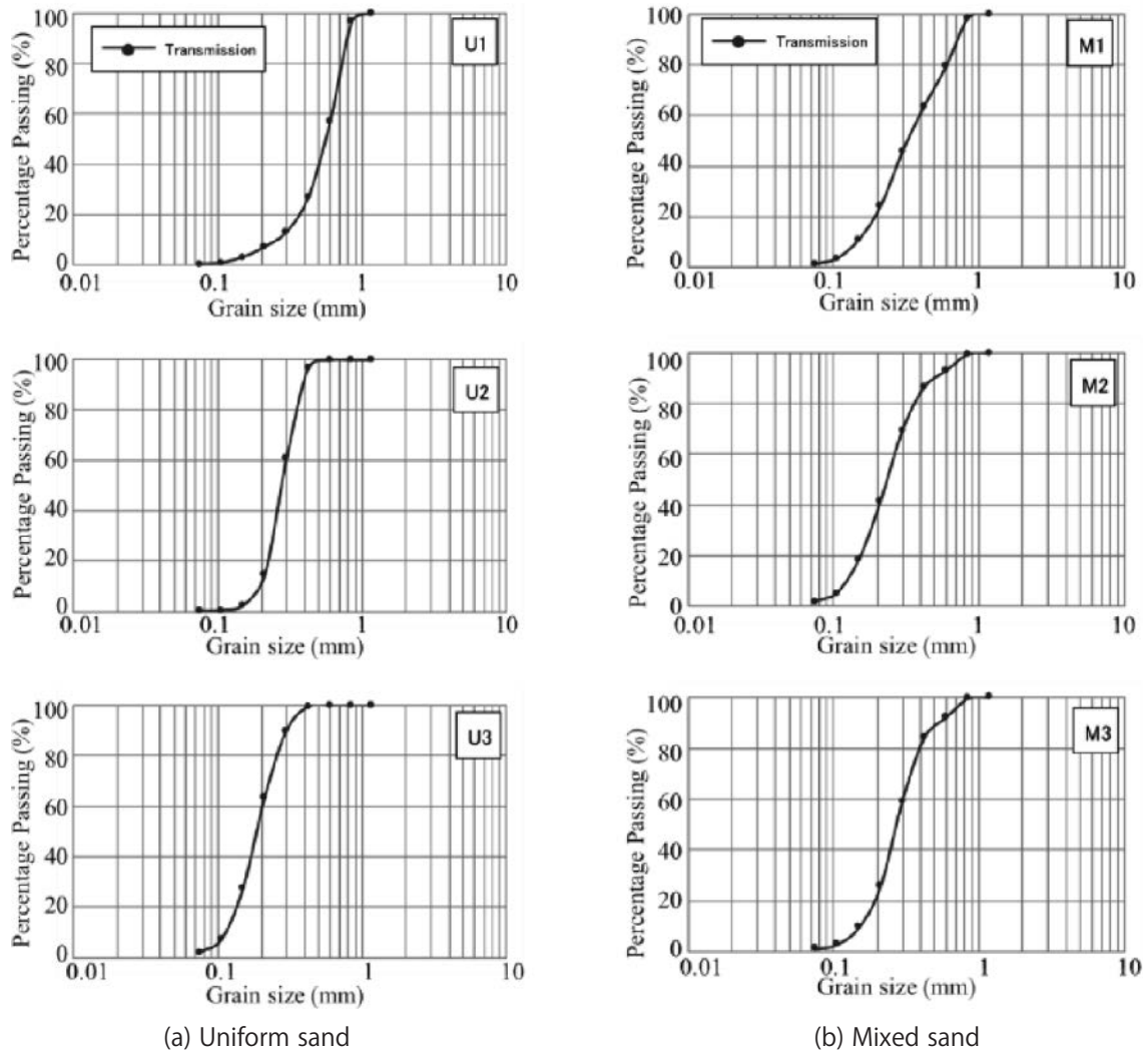
Figure 2. Grain size accumulation curves
