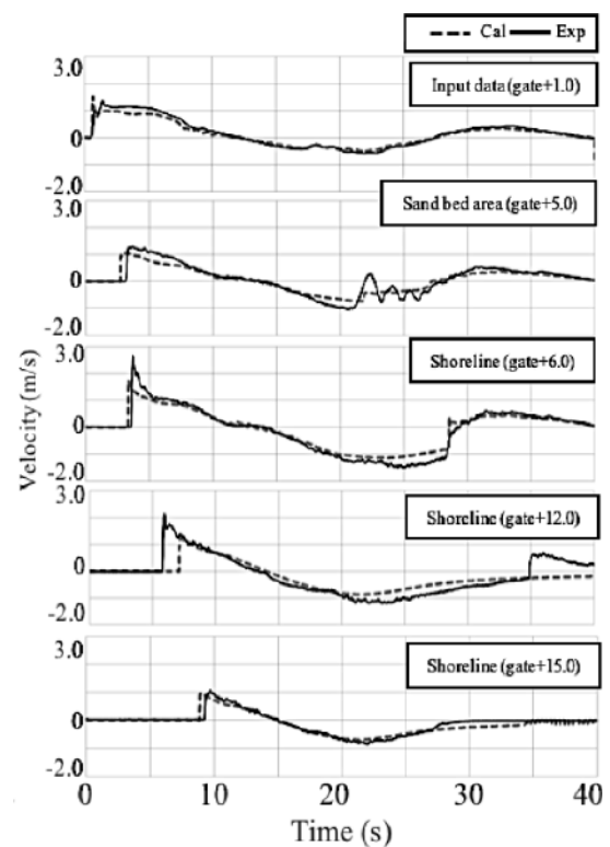
Figure 9. Comparison of velocity at each measurement point with calculation results
