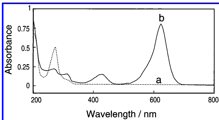
Figure 5. Absorption spectra of crowned Malachite Green 1 (a) before and (b) after UV-light irradiation. [ 1 ]: 1 \times 10^{-5} mol dm -3 in acetonitrile. Photoirradiation: 5 min.
