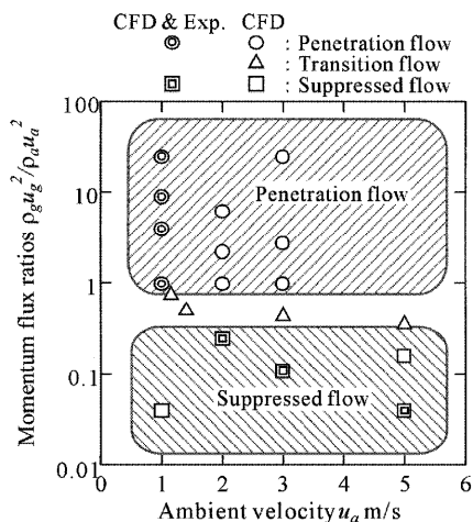
Fig. 10 Flow pattern map of multi-port burner model
