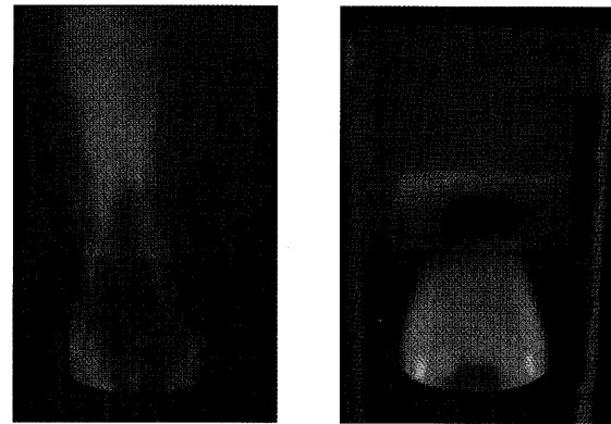
Fig. 6 Flame patterns of DME combustor with co-axial burner D_G/D_P = 4/50 [mm/mm]
