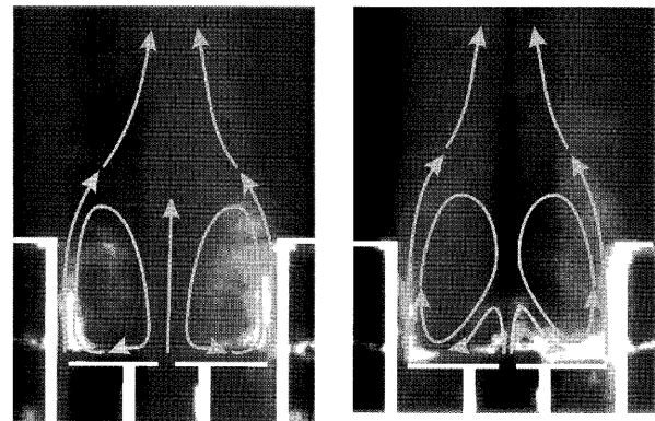
Fig. 7 Flow pattern in co-axial burner model D_G/D_P = 4/50 [mm/mm]
