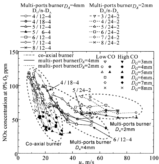
Fig. 12 Relationship between NOx emission and air velocity of DME combustion with multi-port burner, but without water tubes
