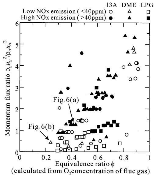
Fig. 5 Relationship between momentum flux ratio and NOx emission in the tube-nested combustor with co-axial burner
