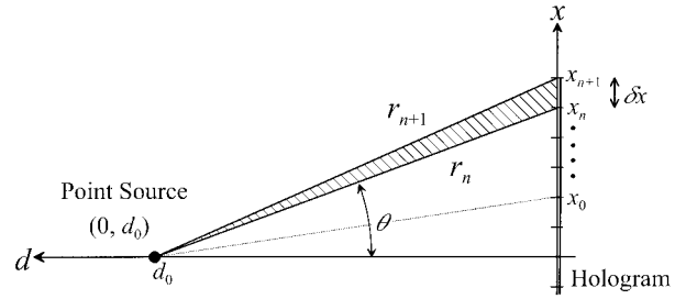
Fig. 2. 2-D coordinates.
