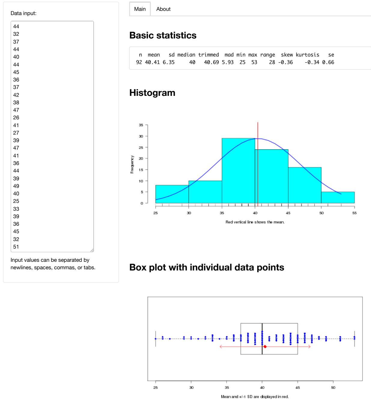
Figure 2. Screenshot of data entry and automatically produced graphics from “langtest.”
