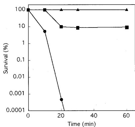
Fig.1 The antimicrobial activity of PAA preparation to E. coli cells. Cells were treated with PAA preparation at 3.5 (closed triangles), 5.0 (closed squares), and 6.9 \mu M (closed circles) at 37 °C.
