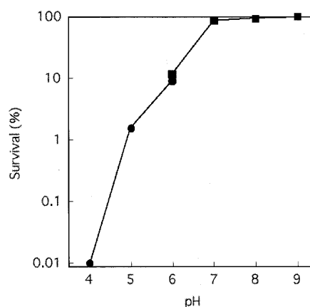
Fig.2 Effect of pHs on the antimicrobial activity of the PAA preparation. Cells were treated with 10.5 \mu M PAA preparation at 37 °C for 5 min. PAA preparations were prepared in 50 mM citrate buffer (closed circles) and potassium phosphate buffer (closed squares).
