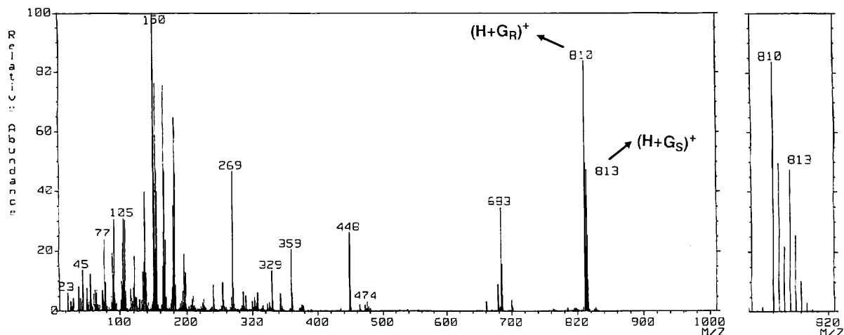
Fig. 3. A FAB mass spectrum (NBA matrix) of chiral crown host 1 (H) with a 1 : 1 mixture of Met-OH·OTs - (G R : G S,d3 ) whose enantiomer is deuterium labeled [( R )-Met-OH - : ( S )-Met(CH 3 S- d 3 )-OH - = 1 : 1]. Peaks at m/z 810 and m/z 813 are the corresponding host-guest complex ions: (H+G R ) + and (H+G S,d3 ) + ions, respectively.
