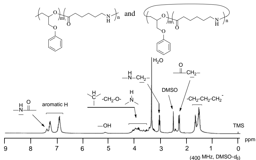
FIGURE 1 ^1\text{H} NMR spectrum of poly( \epsilon -CL- co -GPE).
