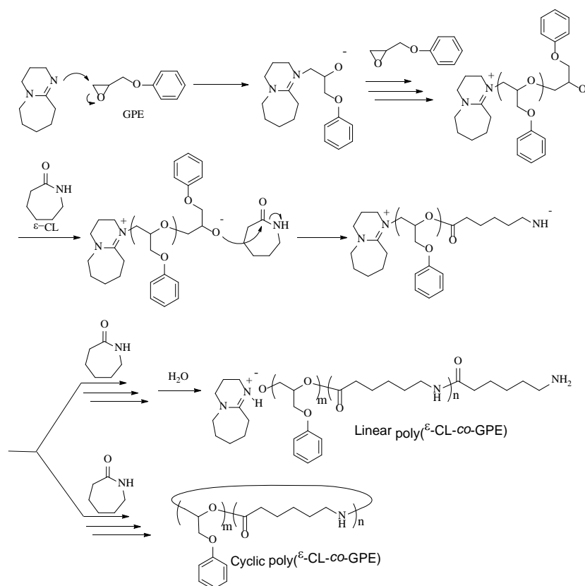
SCHEME 2 Plausible mechanism on the reaction of GPE and \epsilon\text{-CL} with DBU.
