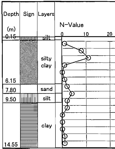
Fig. 2 Geological profile of testing site
