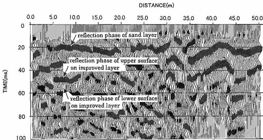
Fig. 6 Time section after improved work in site A (potable vibrator)
