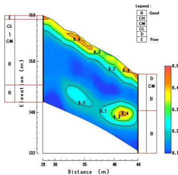
Figure.8-1 Porosity distribution (Aug/2008)
