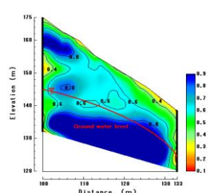
Figure.7-1 Saturation distribution (Aug/2008)
