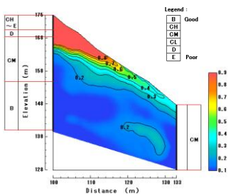
Figure.6-1 Porosity distribution (Aug/2008)
