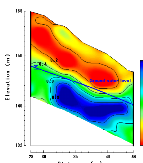
Figure.9-2 Saturation distribution (Dec/2008)
