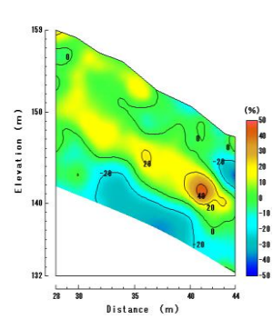
Figure.8-3 Porosity change rate distribution
