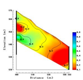
Figure.7-2 Saturation distribution (Dec/2008)
