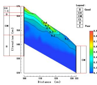
Figure.6-2 Porosity distribution (Dec/2008)
