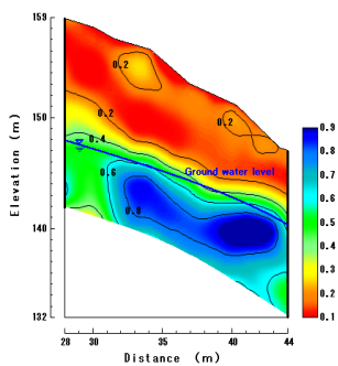
Figure.9-1 Saturation distribution (Aug/2008)
