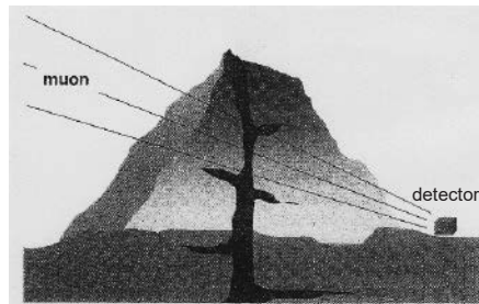
図1 ミュオグラフィの仕組み [3] Fig. 1. Measurement principle of muography. [3]
